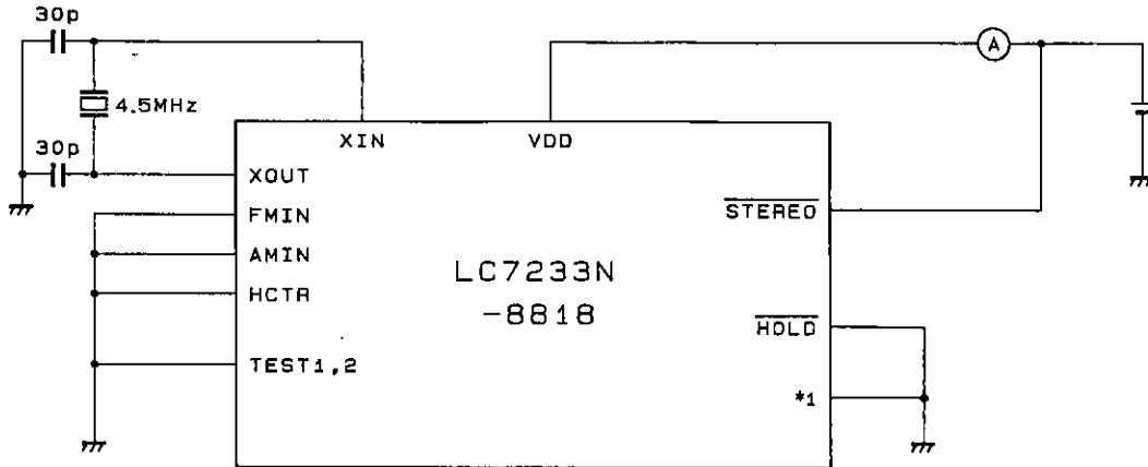
Figure 2 I_{DD3} and I_{DD4} in Backup Mode
