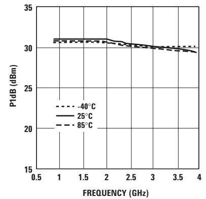
Figure 23. P1dB vs. Temperature and Frequency at optimum P1dB.
