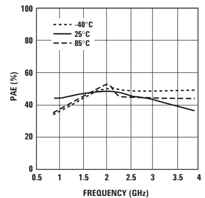
Figure 26. PAE vs. Temperature and Frequency at optimum OIP3.
