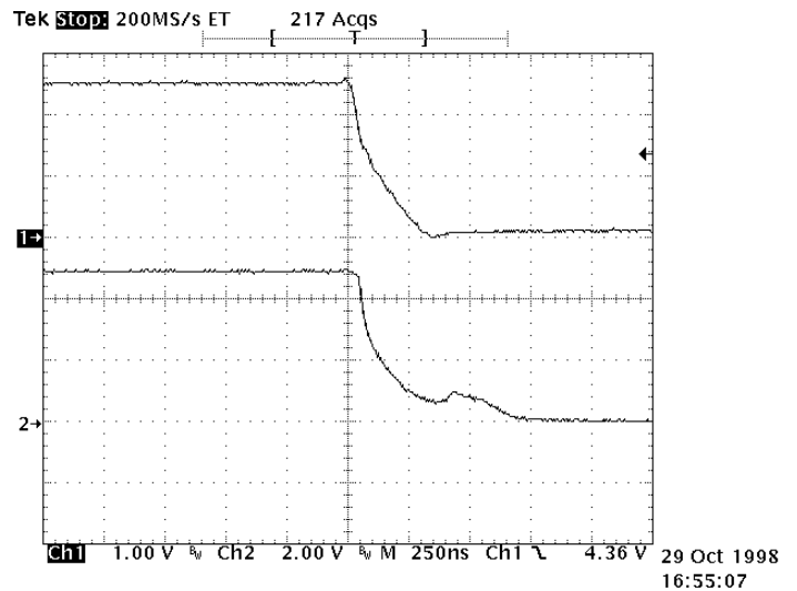
Trace 1: VIN stepping from 5.5V to 3V Trace 2: DR going low at V_{TH(LO)} t_{DL} < 125ns
