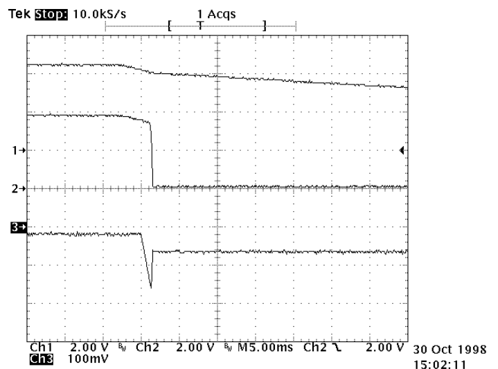
Trace 1: VIN - discharging a 1500uF capacitor Trace 2: DR going low at V_{TH(LO)} Trace 3: VO, offset 3.3V. VO(MIN) = 3.14V
