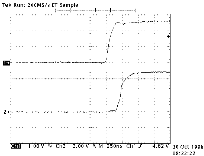
Trace 1: VIN stepping from 3V to 5.5V Trace 2: DR going high at V_{TH(HI)} t_{DH} < 225ns
