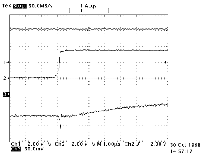
Trace 1: VIN with 3A charging a 1500uF capacitor Trace 2: DR going high at V_{TH(HI)} Trace 3: VO, offset 3.3V. VO(MIN) = 3.19V
