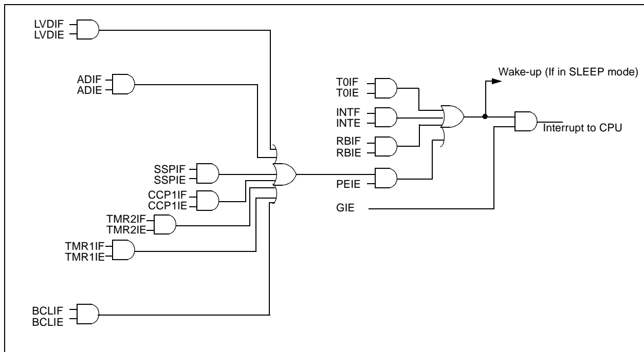
FIGURE 12-11: INTERRUPT LOGIC
