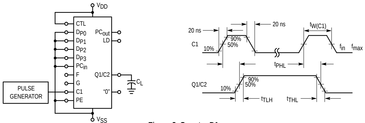
Figure 2. Counter D1
