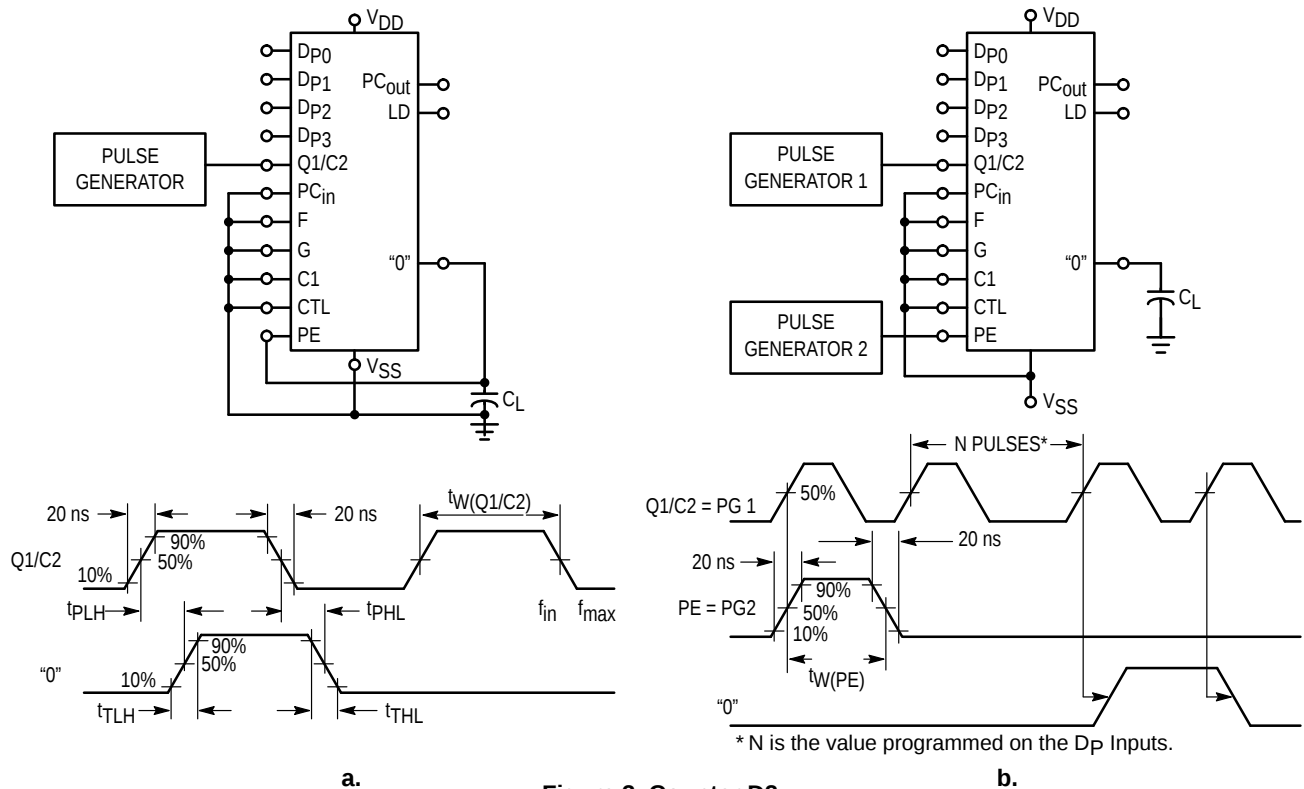
Figure 3. Counter D2
