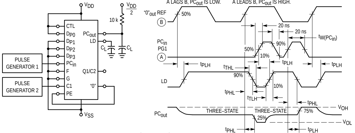
Figure 1. Phase Comparator
