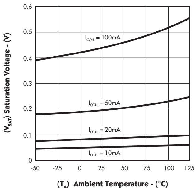
FIGURE 1. — COLLECTOR V_{SAT} vs. TEMPERATURE vs. CURRENT
