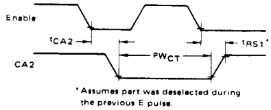
FIGURE 7 — CA2 DELAY TIME (Read Mode; CRA-5=CRA3=1, CRA-4=0)
