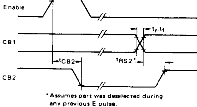
FIGURE 12 — CB2 DELAY TIME (Write Mode; CRB-5=1, CRB-3=CRB-4=0)
