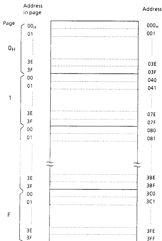
Figure 2-1. Configuration of Program Memory
