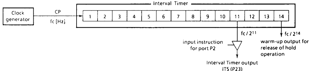
Figure 3-7. Interval Timer
