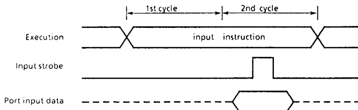
Figure 3-5. Input Timing
