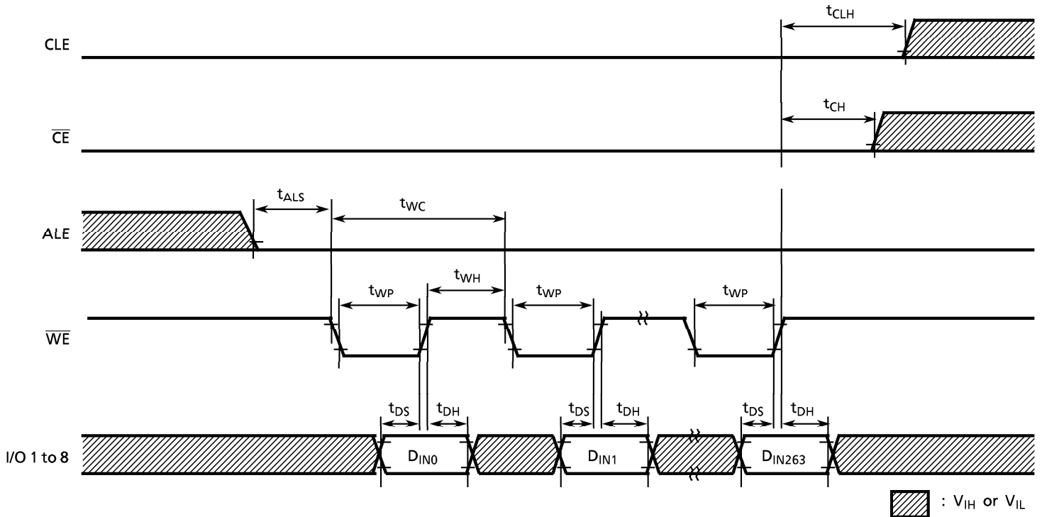
Data Input Cycle Timing Diagram
