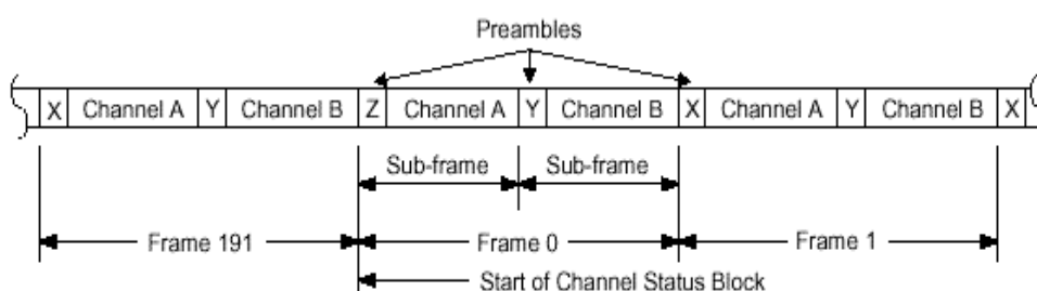
Figure 2. Frame/Block Format
