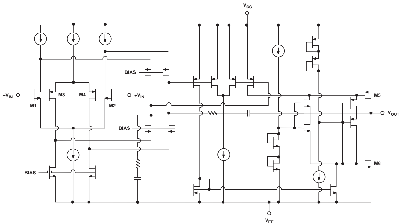
Figure 27. OPx50 Simplified Schematic
