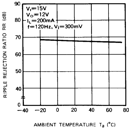
RIPPLE REJECTION RATIO VS. AMBIENT TEMPERATURE
