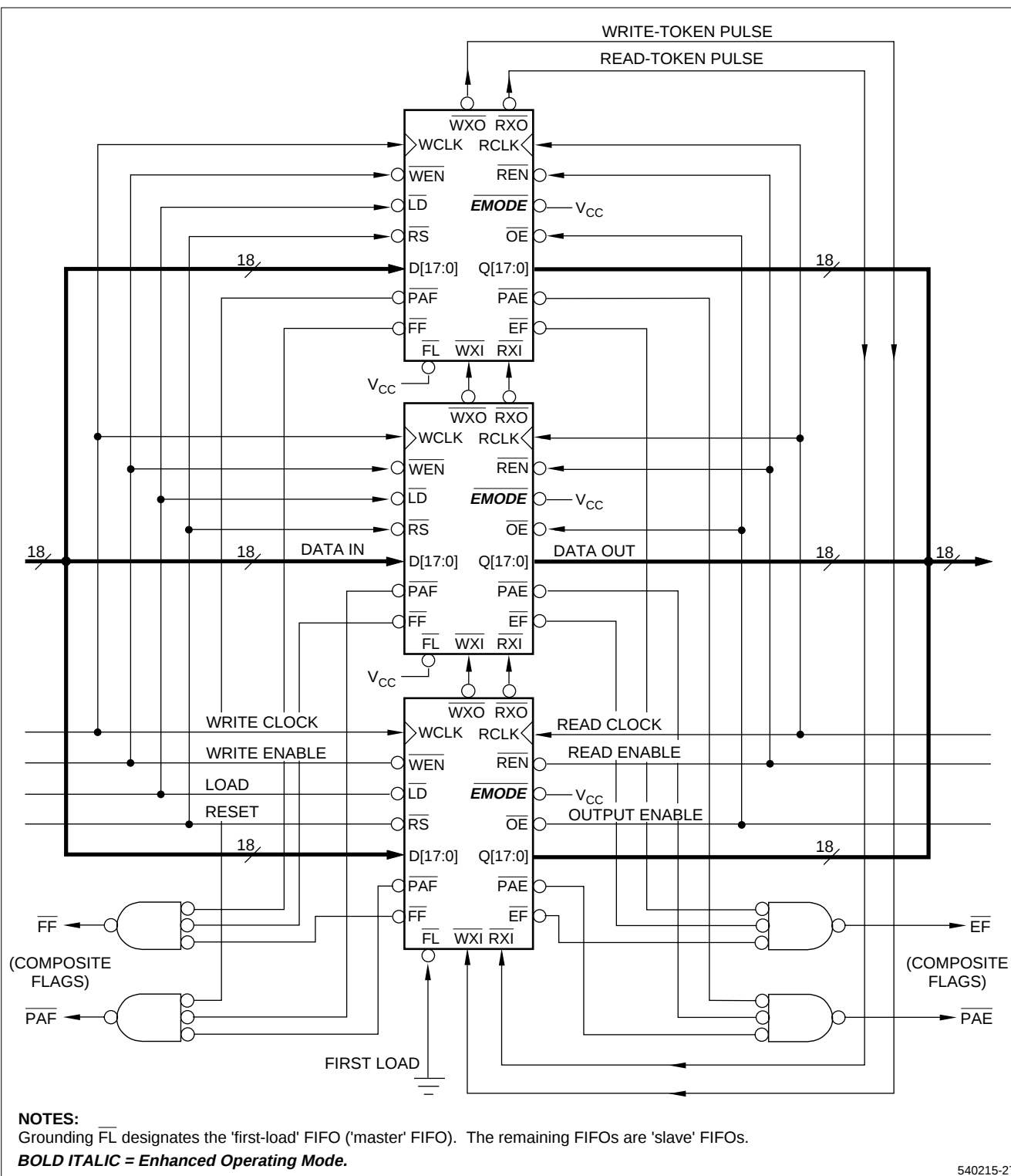
Figure 28. Synchronous-FIFO Depth-Cascading Using IDT-Compatible 'Token-Passing' Scheme
