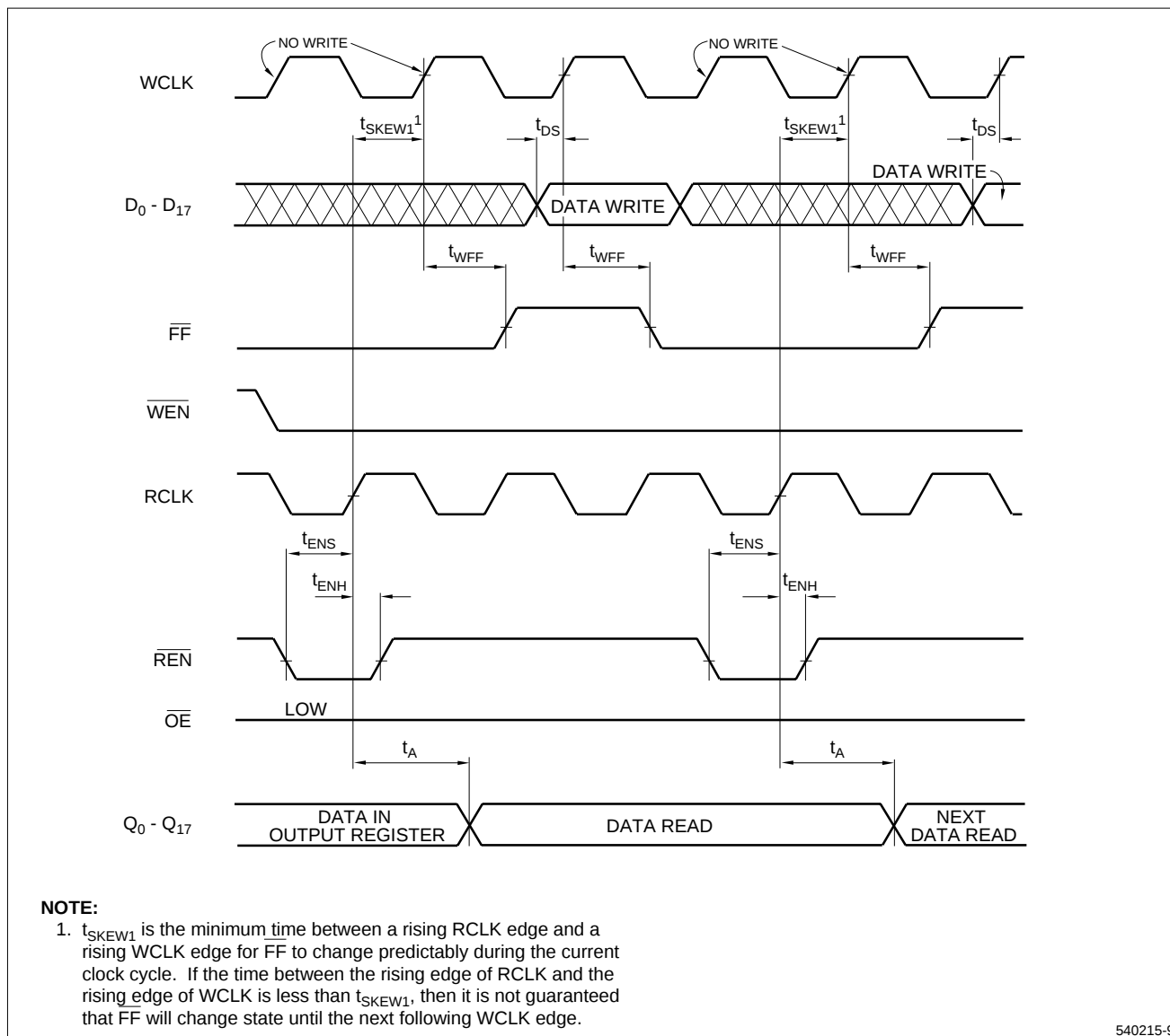
Figure 10. Full-Flag Timing
