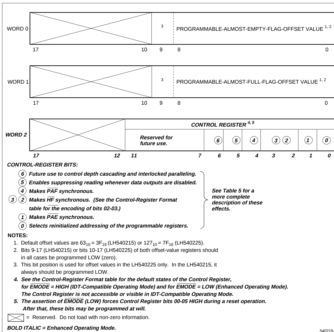
Figure 5. Programmable Registers
