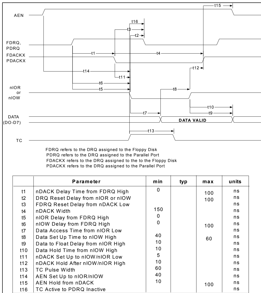
FIGURE 6 - DMA TIMING
