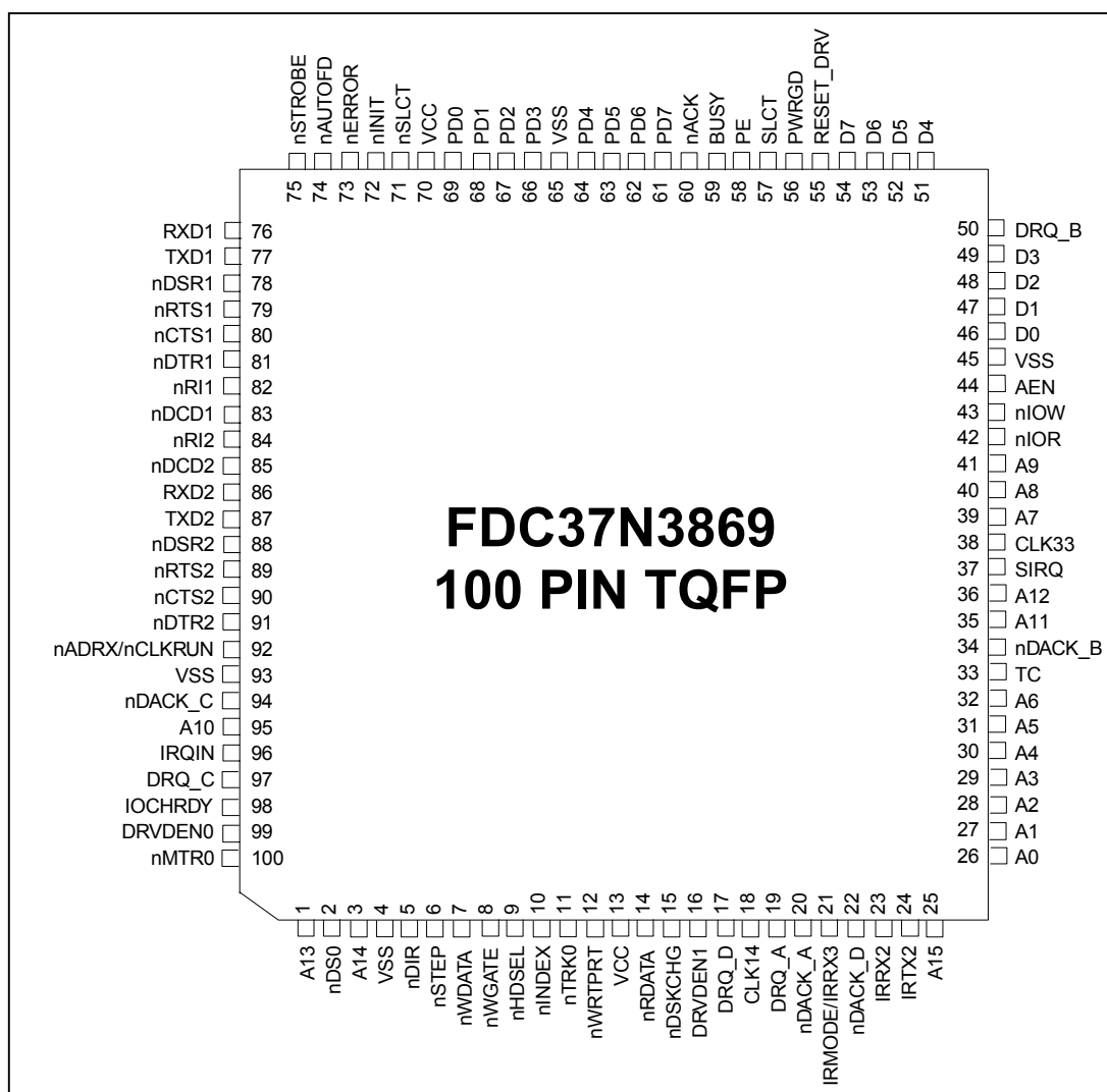
FIGURE 1 - FDC37N3869 PIN CONFIGURATION
