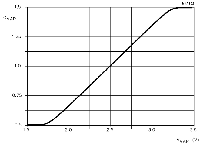
Fig.10 Variable gamma setting as a function of VARGAM setting in sleep mode.
