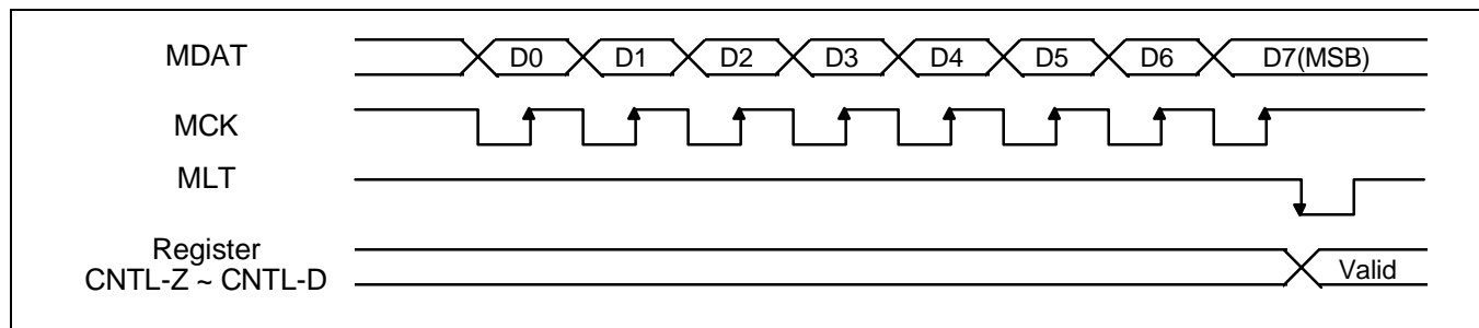
Figure 3. MICOM Data Input Timing Chart
