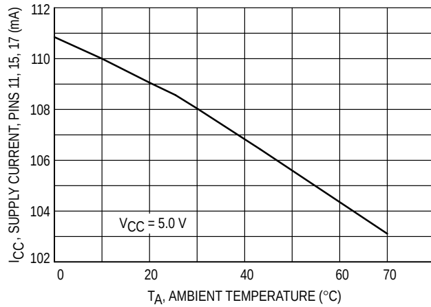
Figure 10. Supply Current versus Temperature
