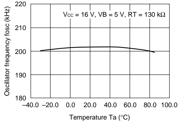
Triangular wave oscillator frequency vs. Temperature characteristics
