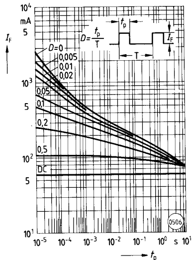
Figure 17. Permissible pulse load D =parameter, T_A=25^\circ\text{C} , I_F=f(t_p)
