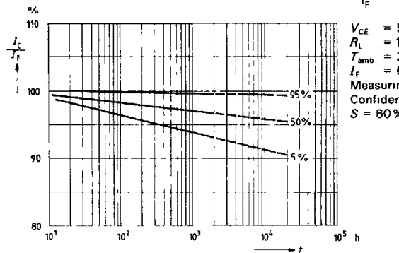
Variation of current transfer ratio as a function of load time
