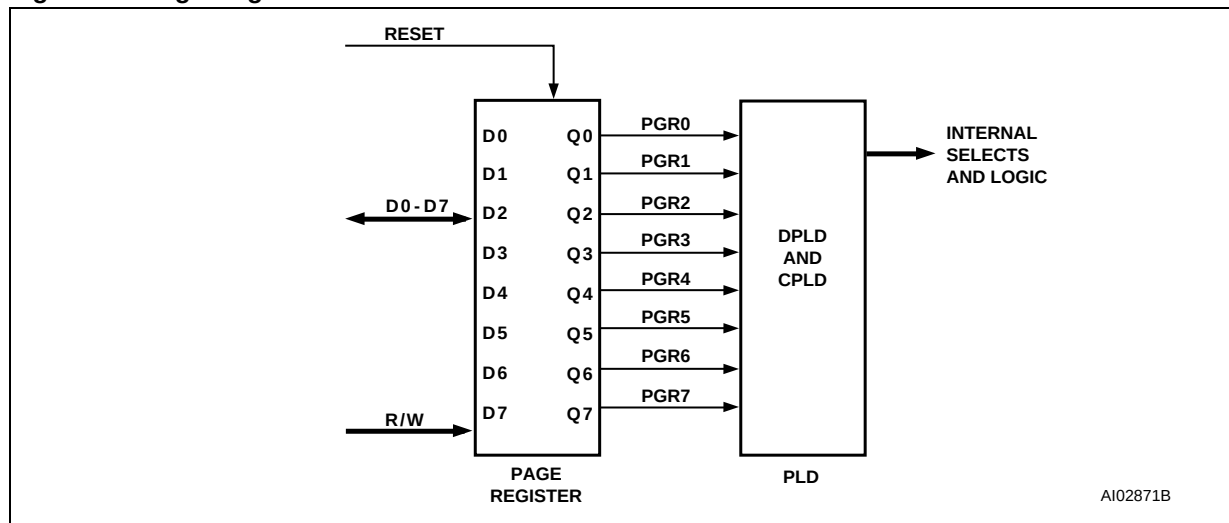
Figure 10. Page Register
