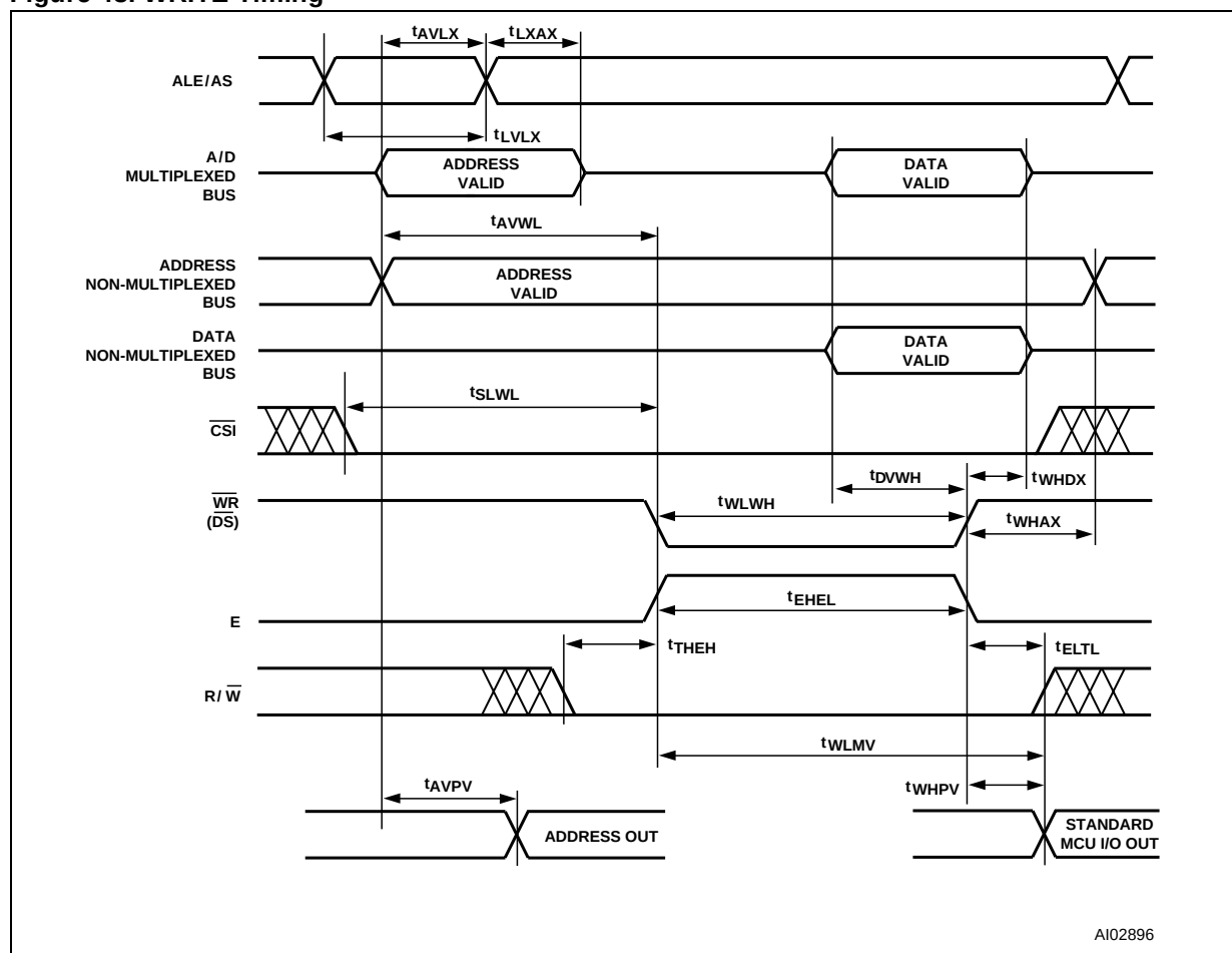
Figure 43. WRITE Timing
