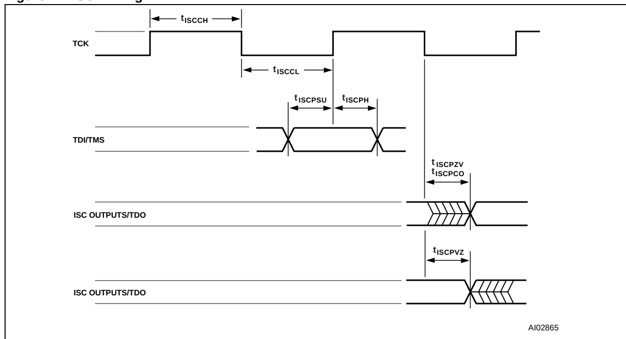
Figure 47. ISC Timing
