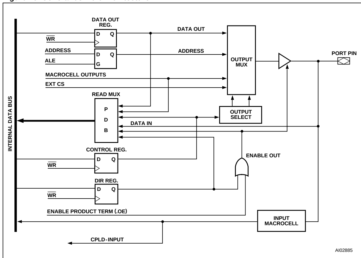
Figure 23. General I/O Port Architecture
