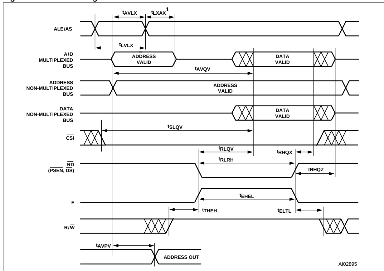
Figure 42. READ Timing
