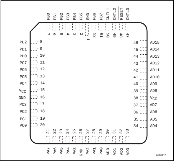
Figure 49. PLCC52 Connections
