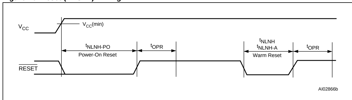
Figure 46. Reset (RESET) Timing
