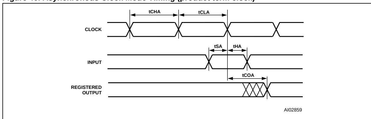
Figure 40. Asynchronous Clock Mode Timing (product term clock)
