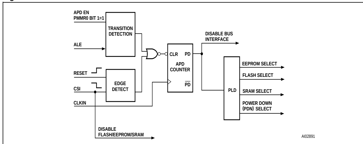
Figure 29. APD Unit
