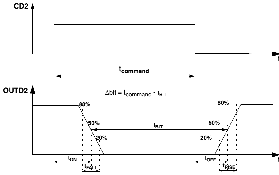
Figure 2. Timing Characteristics
