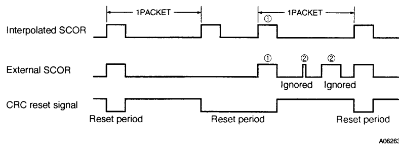
Figure 4 Synchronizing Signal Interpolation and Protection
