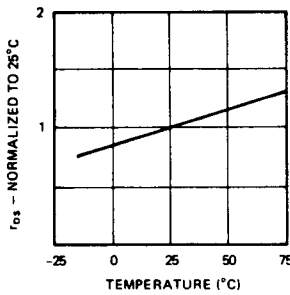
r_{DS(ON)} vs TEMPERATURE (Normalized to 25 ^{\circ} C Value)
