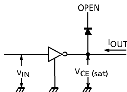
2. V_{CE(sat)}
