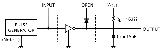
8. t_{ON}, t_{OFF}
