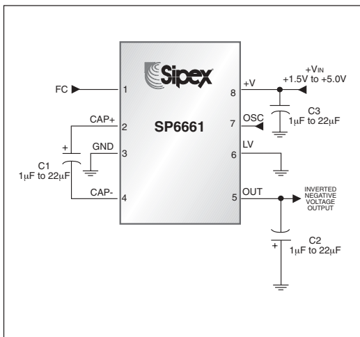
Figure 1: Voltage Inverter
