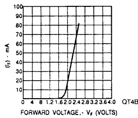
FIGURE 3: MAN5750/MAN5760
