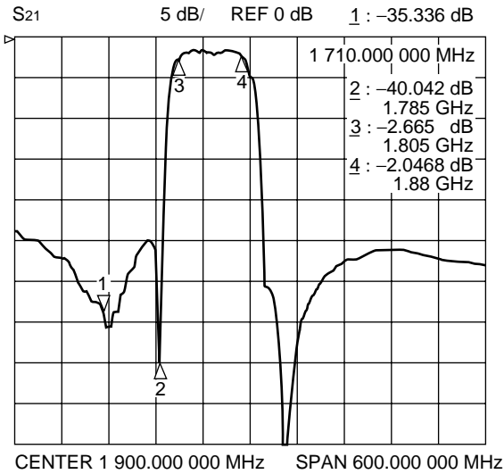
Filter 1 (Passband : 1805 to 1880 MHz)
