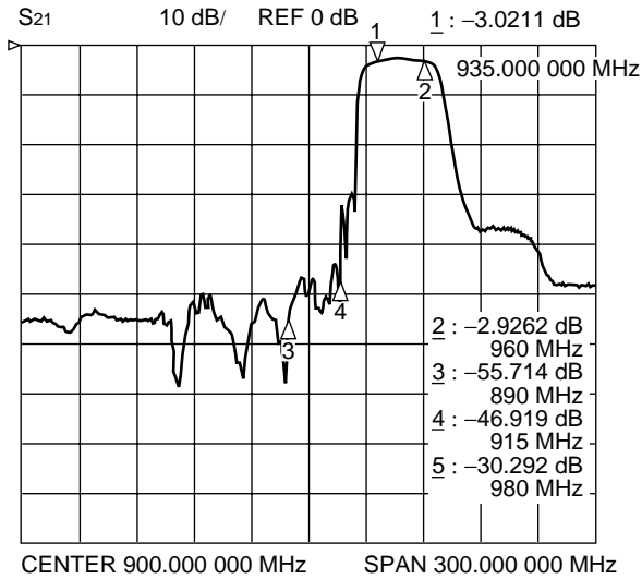
Filter 1 (Passband : 935 to 960 MHz)
