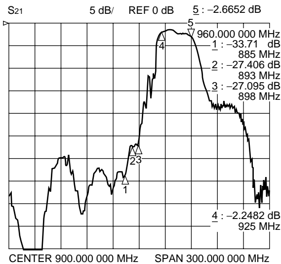
Filter 2 (Passband : 925 to 960 MHz)
