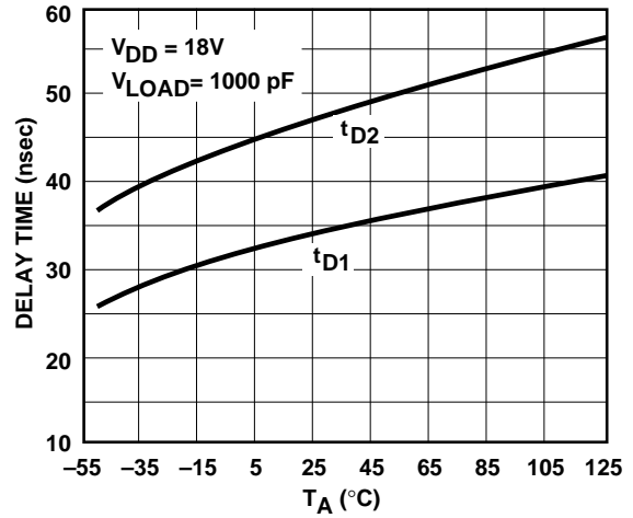
Propagation Delay Time vs. Temperature
