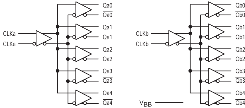
Figure 2. Logic Symbol
