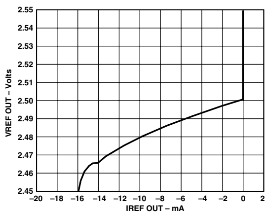
Figure 31. Reference Voltage vs. Reference Load
