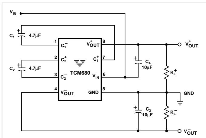
Figure 1. Test Circuit
