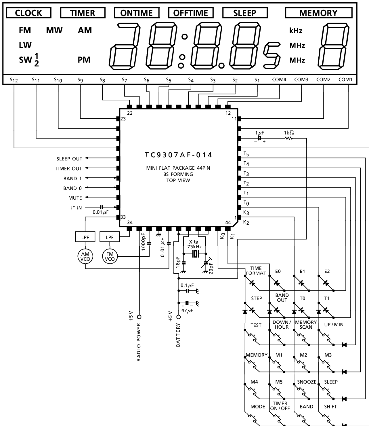
TC9307AF-014 Layout
