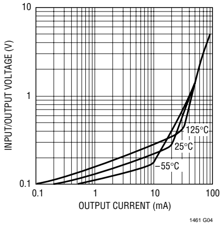
Minimum Input/Output Voltage Differential vs Load Current
