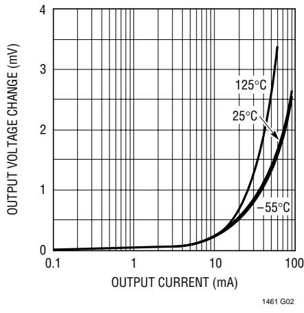
Load Regulation
