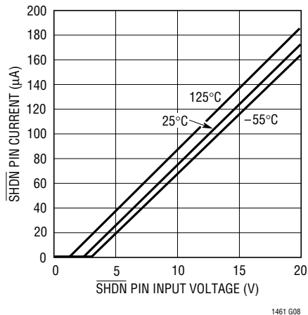
SHDN Pin Current vs SHDN Input Voltage
