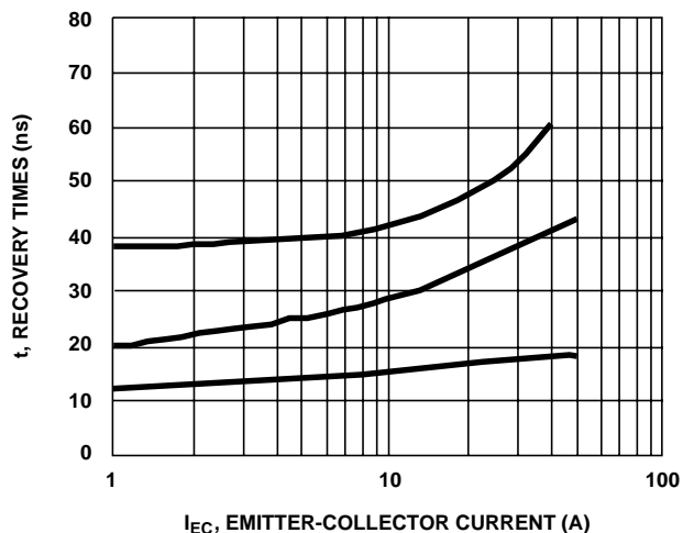
FIGURE 12. TYPICAL t_{RR} , t_A , t_B vs FORWARD CURRENT
