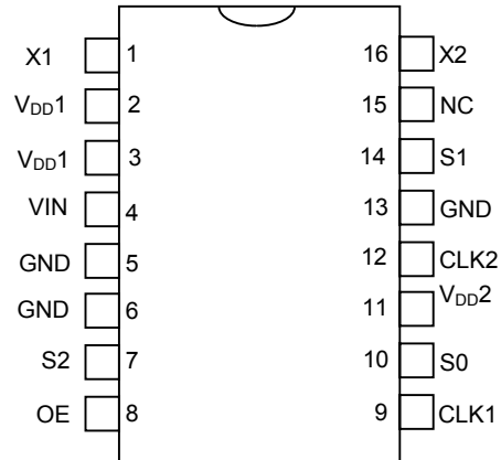
VT83205 Pinout
