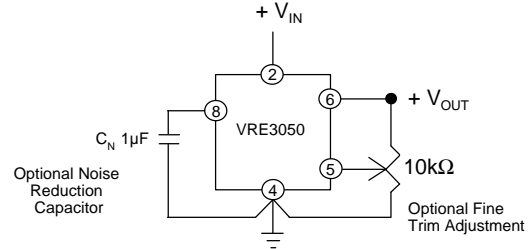
Figure 3 External Connections
