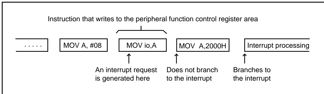
Figure 6.4-1 Hardware interrupt request while writing to the peripheral function control register area
