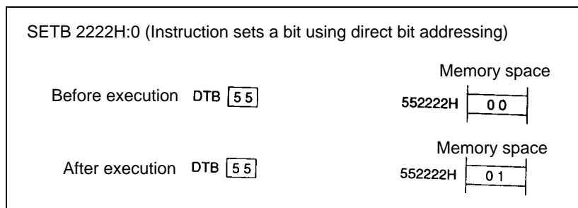
Figure B.3-10 Example of direct bit addressing (addr16:bp)
