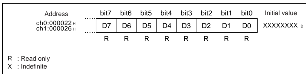
Figure 13.4-5 Serial input data register (SIDR0/1)
