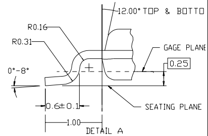
14-Lead Thin Shrink Small Outline Package (TSSOP), JEDEC MO-153, 4.4mm Wide Package MTC14
