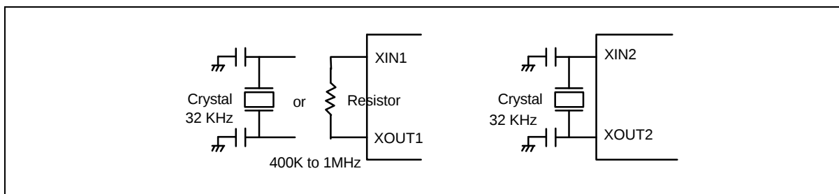
Figure 3. Oscillator Configuration
