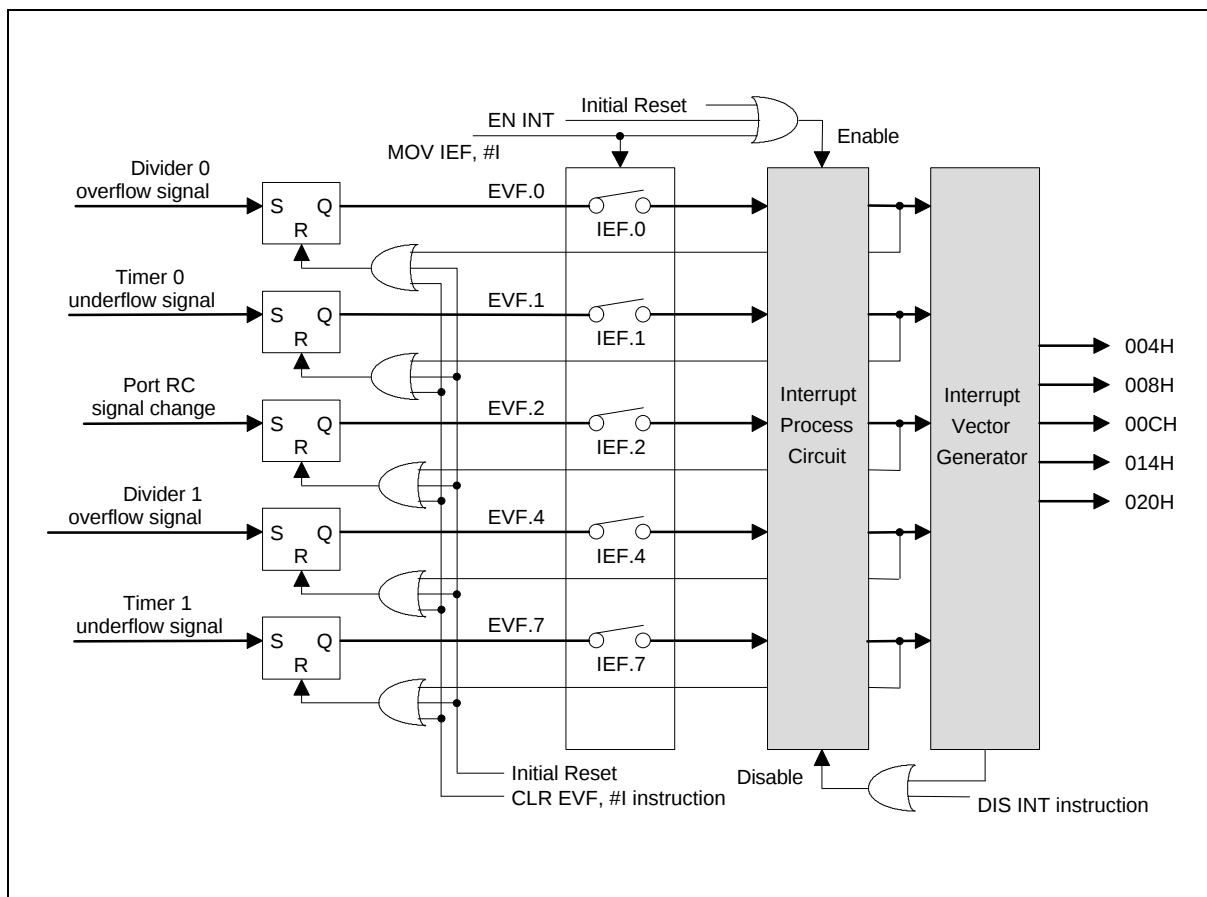
Figure 7. Interrupt Event Control Diagram
