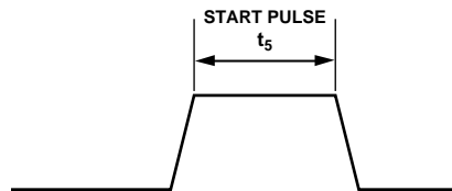
Figure 3. Daisy-Chain Start Timing
