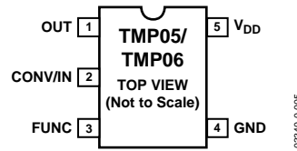
Figure 5. Pin Configuration
