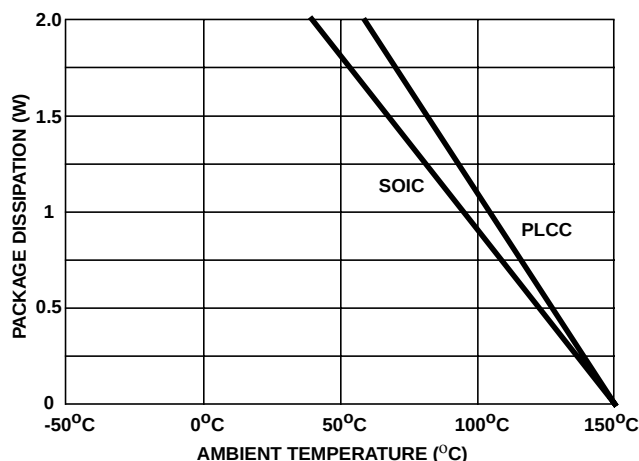
FIGURE 6. MAXIMUM POWER DISSIPATION RATING vs TEMPERATURE FOR THE CA3272AQ, CA3292AQ PLCC PACKAGE AND THE CA3272AM, CA3292AM SOIC PACKAGE WITH NO ADDITIONAL PC BOARD AREA FOR HEAT SINKINGS
