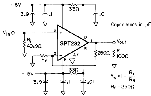
Figure 1: suggested non-inverting gain circuit
