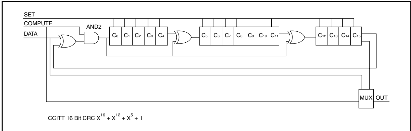
FIGURE 3: CCITT TYPE
