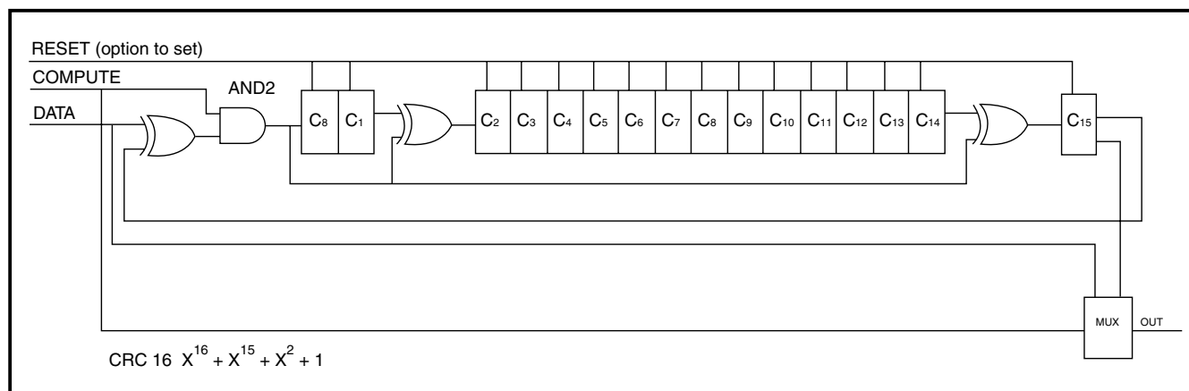
FIGURE 4: CRC 16
