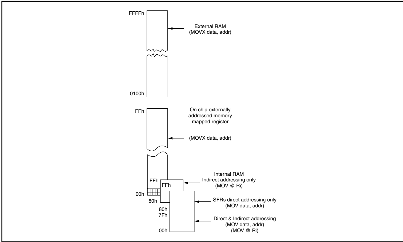
FIGURE 6: Memory Map
