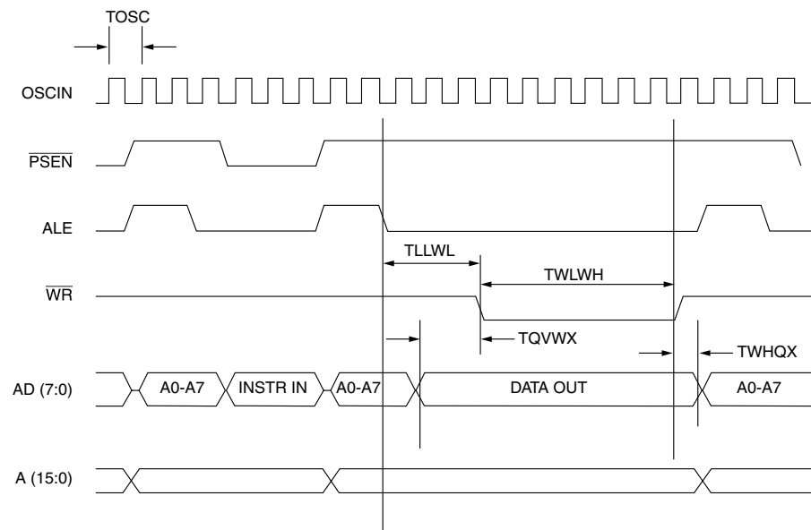
FIGURE 11: External Data Memory Write Cycle
