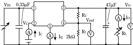
Fig. 1 Test Circuit
