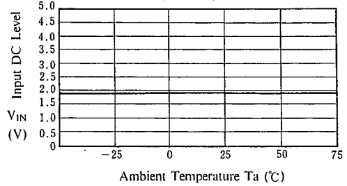
Input DC Level vs. Ta ( V^+ = 5V )
