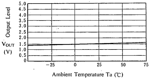
Output DC Level vs. Ta ( V^+ = 5V )
