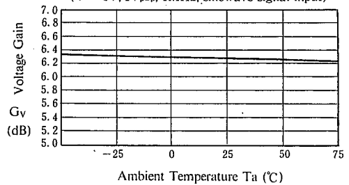
Voltage Gain vs. Ta (Clamp Type INput) ( V^+ = 5V, 1V_{p-p}, 1MHz, \text{sinewave signal input} )
