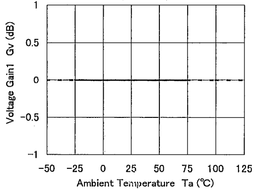
Voltage Gain1 vs. Temperature ( f=100\text{kHz} )
