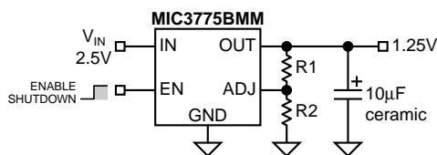
1.25V/750mA Adjustable Regulator
