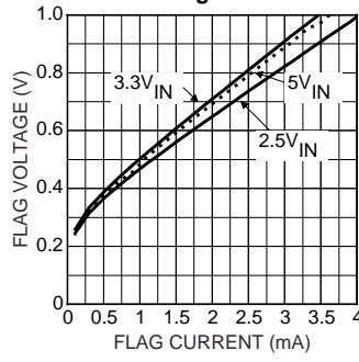
Flag Voltage vs. Flag Current
