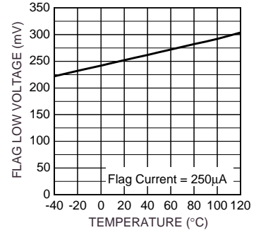
Flag Low Voltage vs. Temperature
