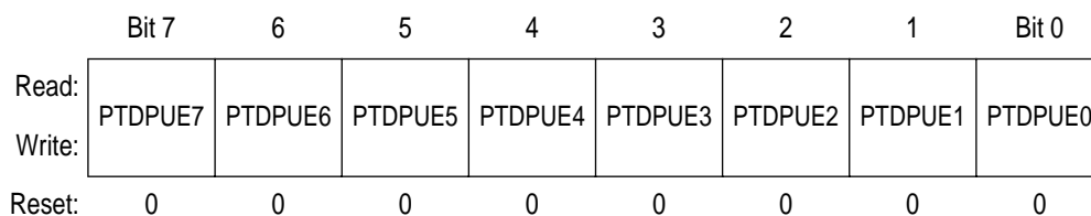
Figure 17-14. Port D Input Pullup Enable Register (PTDPUE)
